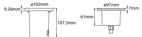
Housing (incluido)
